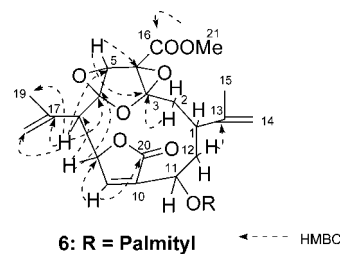
Figure 2. 1 H- 13 C HMBC correlations of 6 .
